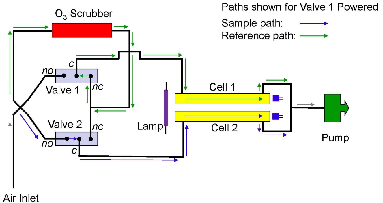
Figure 1-1. Schematic diagram of the Model 205 Dual Beam Ozone Monitor.
